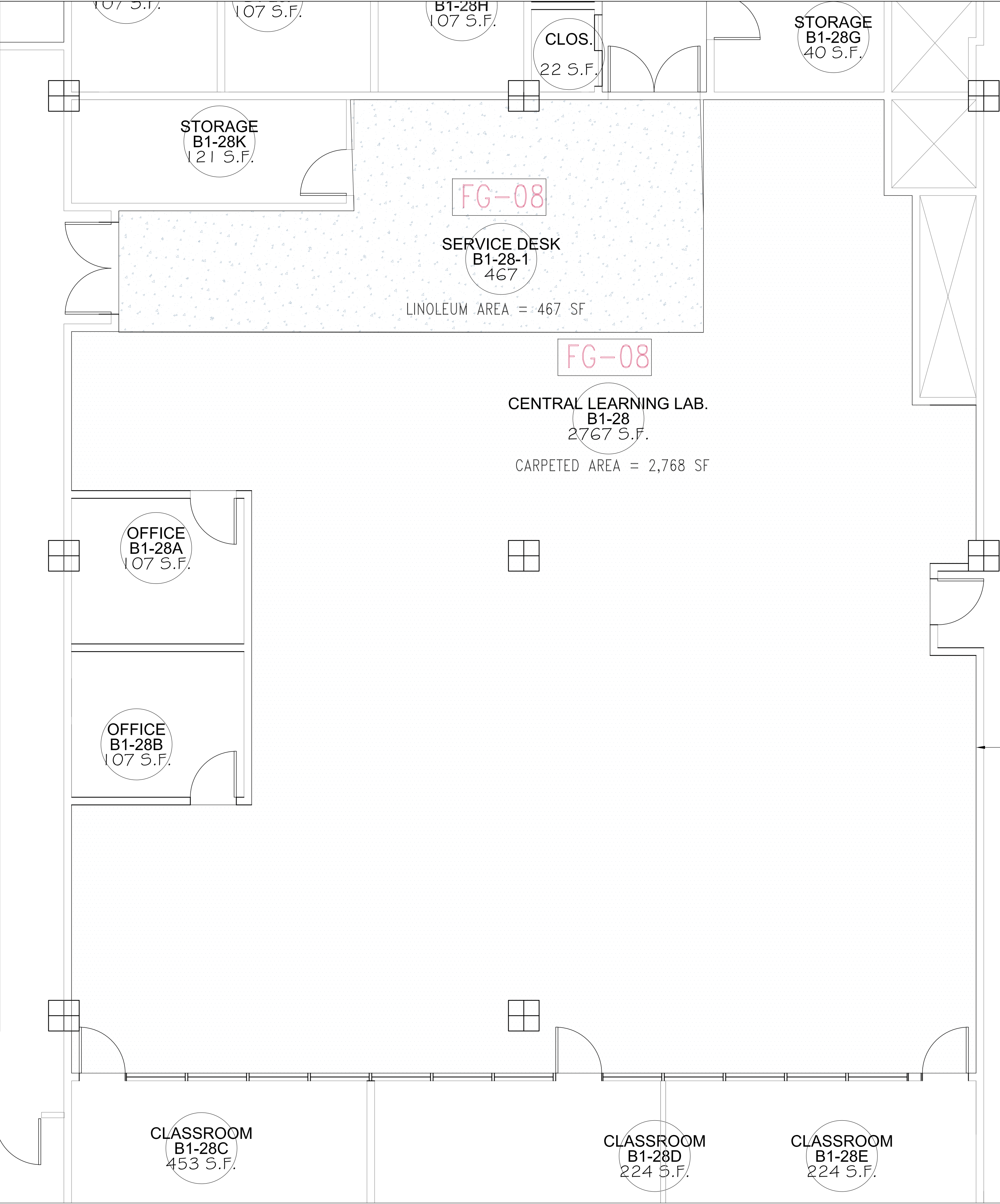
2 FINISH PLAN: B1-28, LEARNING LAB SCALE: 1/4" = 1'-0"
